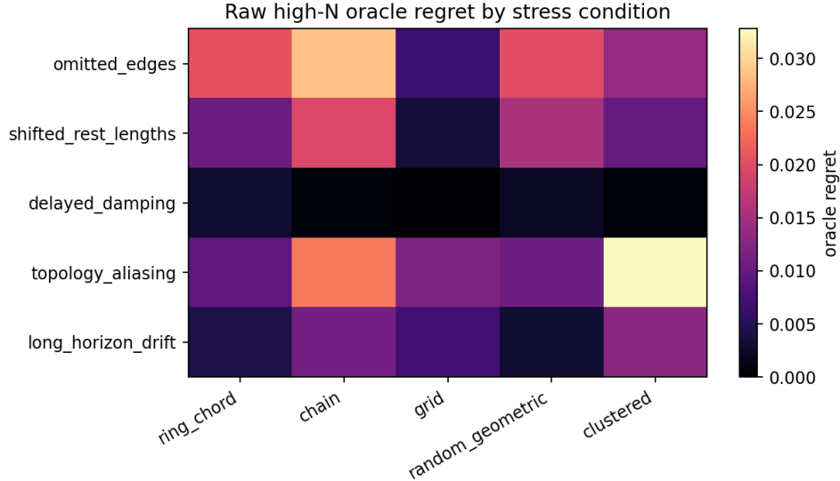
Figure 2: raw N = 64 oracle regret across graph families and hidden-failure modes in the stress suite.
